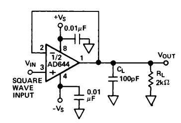
Figure 21c. Unity Gain Follower
