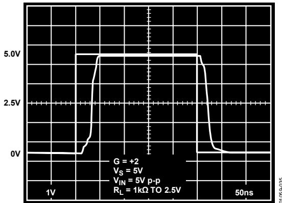
Figure 35. Overdrive Recovery
