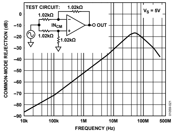
Figure 21. Common-Mode Rejection (CMR) vs. Frequency
