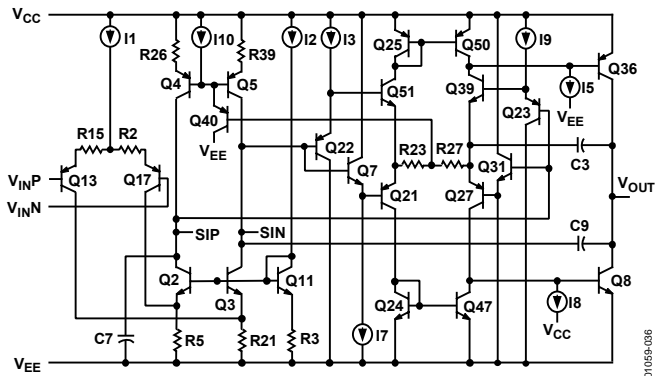
Figure 36. Simplified Schematic
