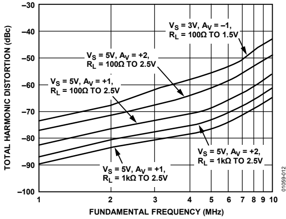
Figure 12. Total Harmonic Distortion
