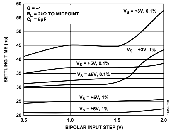
Figure 20. Settling Time
