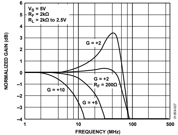
Figure 27. Frequency Response vs. Closed-Loop Gain
