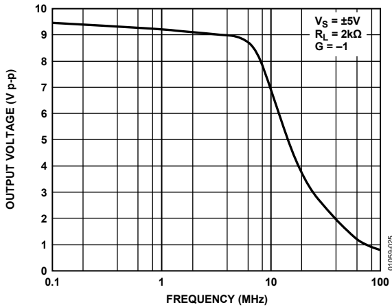
Figure 25. Output Voltage Swing vs. Frequency
