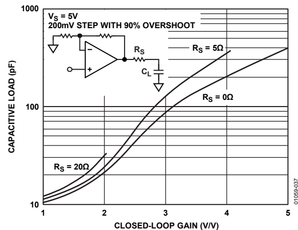
Figure 37. Capacitive Load Drive vs. Closed-Loop Gain
