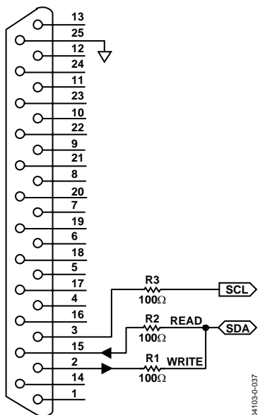
Figure 47. Parallel Port Connection. Pin 2 = SDA_write, Pin 3 = SCL, Pin 15 = SDA_read, and Pin 25 = DGND.
