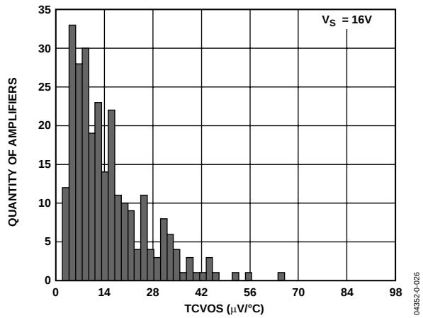
Figure 3. Input Offset Voltage Drift, V_S = 16V
