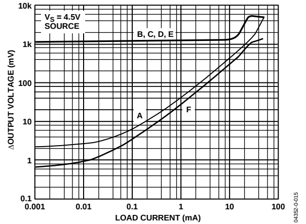
Figure 7. Output Source Voltage vs. Load Current, All Channels
