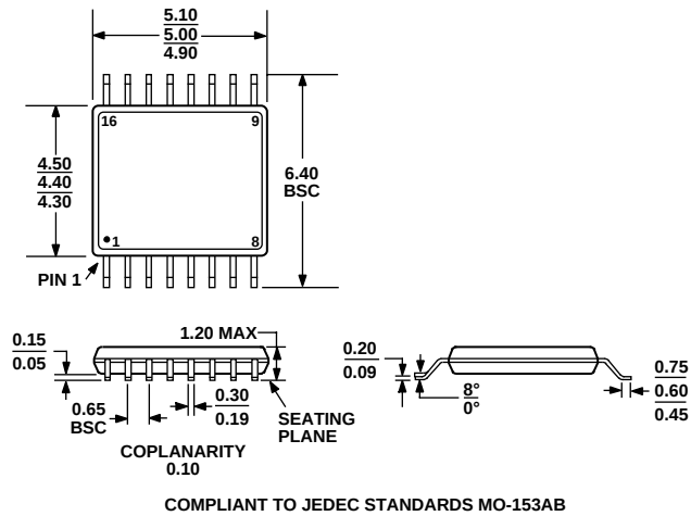
Figure 22. 16-Lead Thin Shrink Small Outline Package [TSSOP] (RU) Dimensions shown in millimeters
