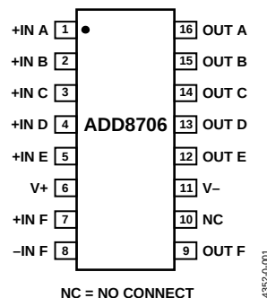
Figure 1. 16-Lead TSSOP
