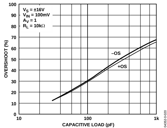
Figure 17. Overshoot vs. Capacitive Load
