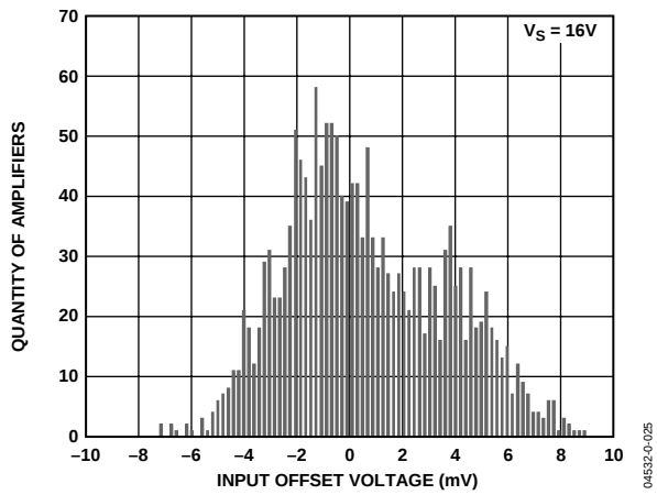
Figure 2. Input Offset Voltage, V_S = 16V
