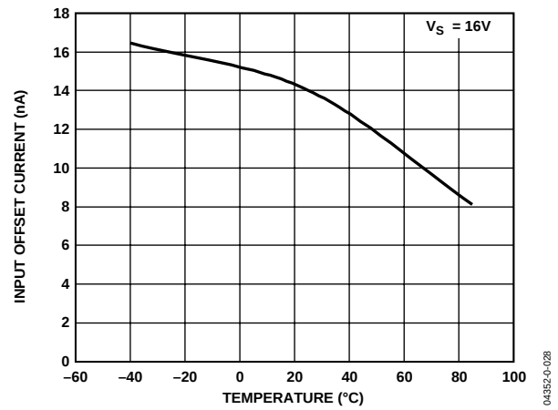
Figure 5. Input Offset Current vs. Temperature
