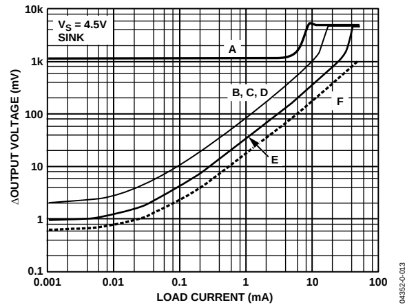
Figure 6. Output Sink Voltage vs. Load Current, All Channels
