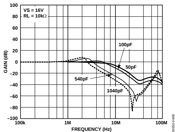
Figure 15. Gain vs. Capacitive Load
