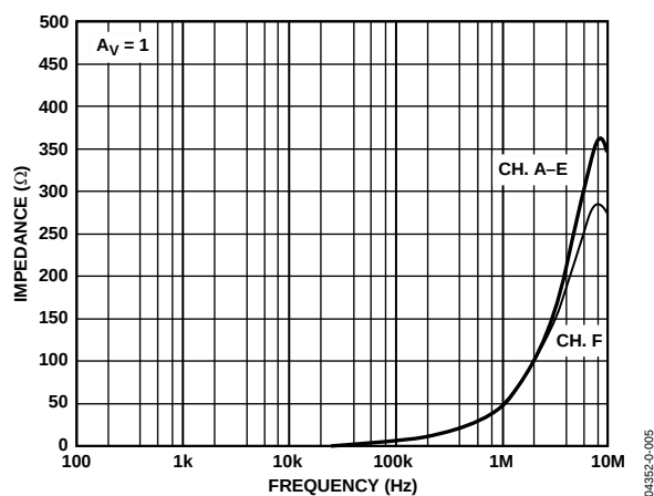
Figure 16. Impedance vs. Frequency
