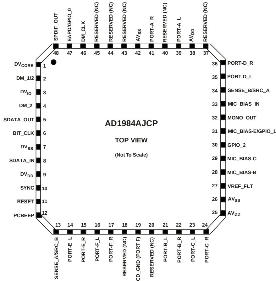
Figure 2. AD1984A 48-Lead Package and Pinout
