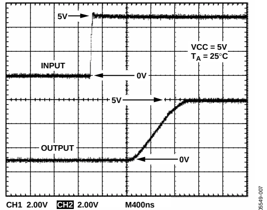
Figure 10. Transient Response—Rising
