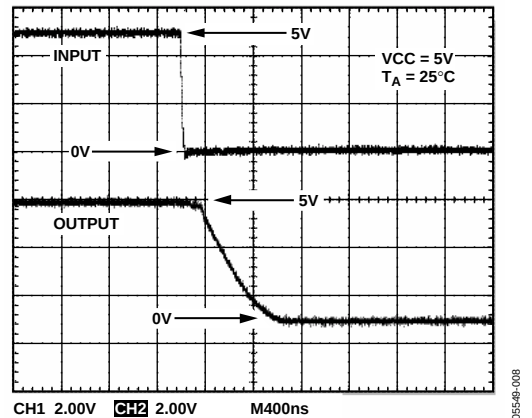
Figure 11. Transient Response—Falling
