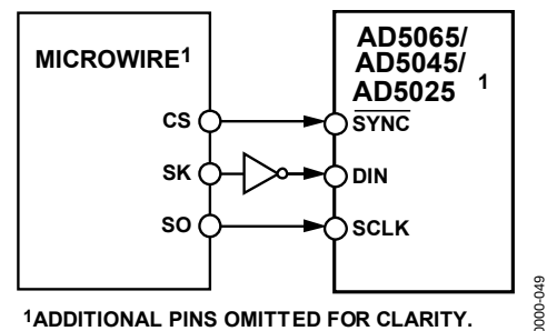
Figure 51. AD5025/45/65 to MICROWIRE Interface
