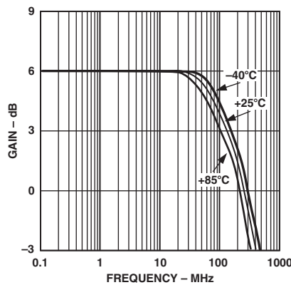
TPC 11. Frequency Response vs. Temperature, Gain = +2, V_S = \pm 5\text{ V} , V_{OUT} = 2\text{ V p-p}
