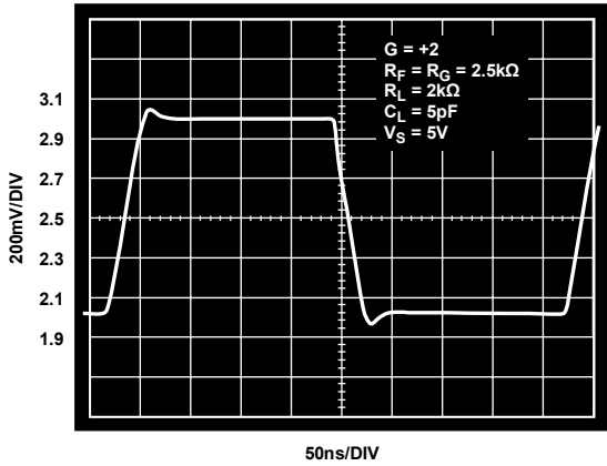
Figure 39. 1 V Step Response
