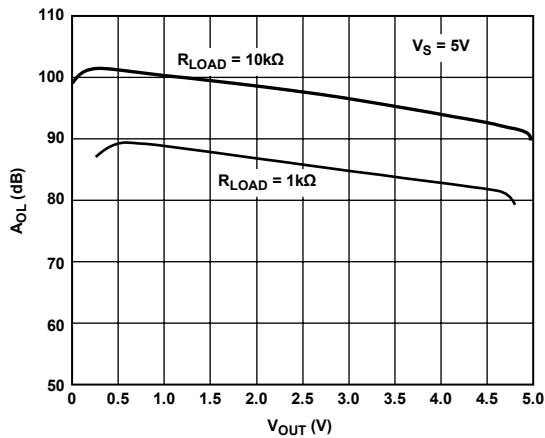
Figure 22. Open-Loop Gain ( A_{OL} ) vs. V_{OUT}
