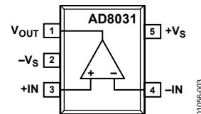
Figure 3. 5-Lead SOT-23 (RJ-5)
