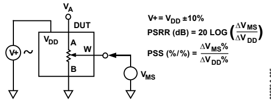
Figure 28. Test Circuit for Power Supply Sensitivity (PSS, PSSR)
