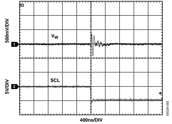
Figure 28. Digital Feedthrough
