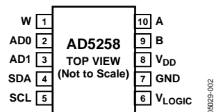
Figure 3. Pinout
