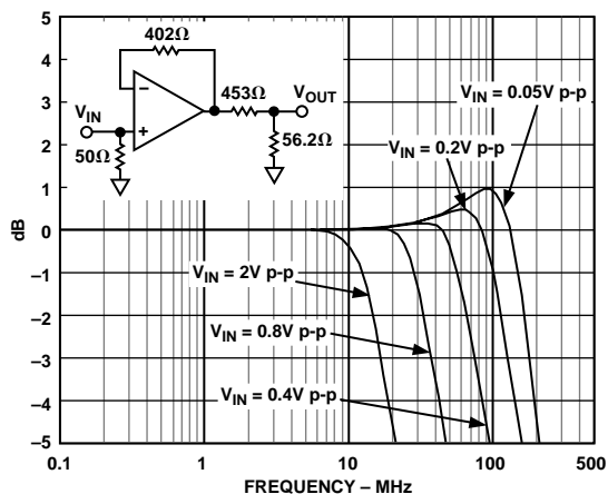
Figure 3. Frequency Response vs. Signal Level, V_S = \pm 12 V , G = 1
