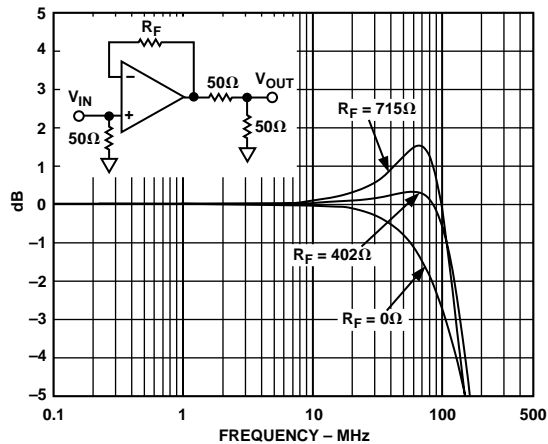
Figure 6. Frequency Response vs. R_F , G = 1 , V_S = \pm 12 V , V_{IN} = 22 \text{ dBm}
