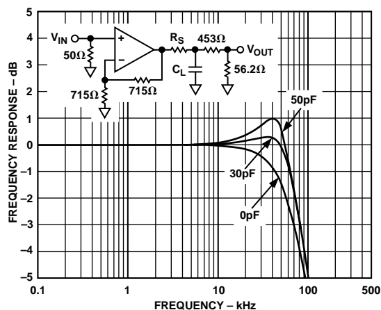
Figure 30. Frequency Response vs. Capacitive Load, C_L = 0\text{ pF} , 30\text{ pF} and 50\text{ pF} , R_S = 0\ \Omega
