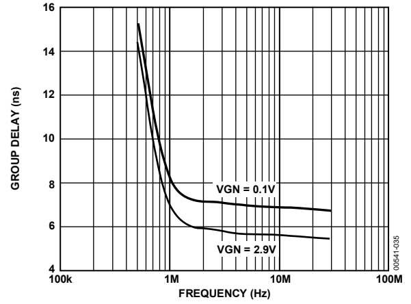
Figure 34. Group Delay vs. Frequency
