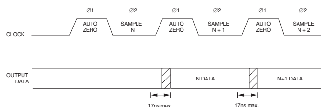
TIMING DIAGRAM
