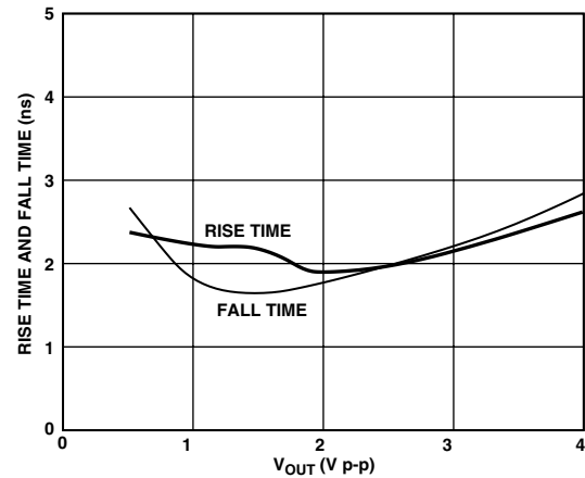
TPC 23. Rise Time and Fall Time vs. V_{OUT} , G = +2 , R_L = 100\text{ }\Omega , R_F = 402\text{ }\Omega
