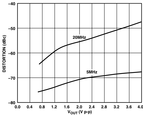
TPC 21. Distortion vs. V_{OUT} @ 20 MHz, 5 MHz, R_L = 150\text{ }\Omega , V_S = \pm 5.0\text{ V}
