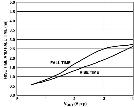
TPC 22. Rise Time and Fall Time vs. V_{OUT} , G = +1 , R_L = 1\text{ k}\Omega , R_F = 0\text{ }\Omega
