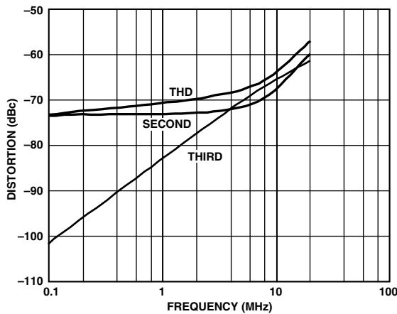
TPC 20. Distortion vs. Frequency, R_L = 150\text{ }\Omega
