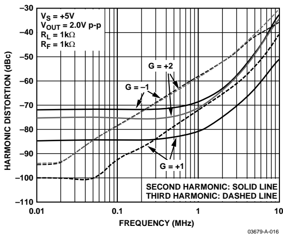
Figure 21. Harmonic Distortion vs. Frequency and Gain
