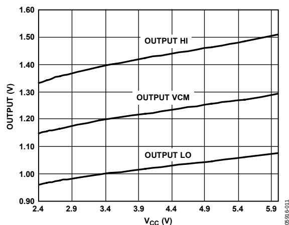
Figure 8. Output Level vs. V_{CC}
