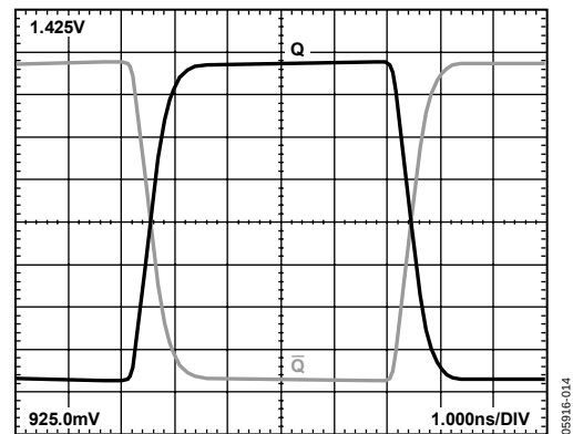
Figure 15. 50 MHz Output Voltage Waveform V CCO = 2.5 V
