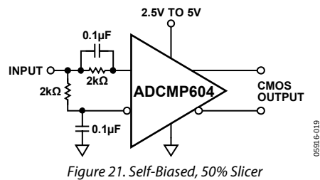
Figure 21. Self-Biased, 50% Slicer
