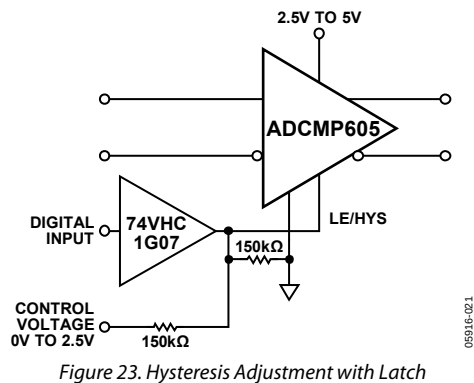
Figure 23. Hysteresis Adjustment with Latch
