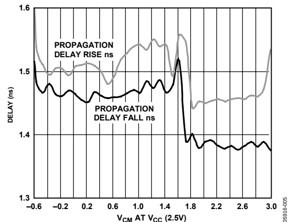
Figure 13. Propagation Delay vs. Input Common Mode
