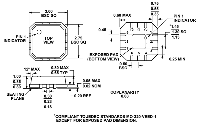
Figure 28. 12-Lead Lead Frame Chip Scale Package (LFCSP-VQ) 3 mm x 3 mm Body, Very Thin Quad (CP-12-1) Dimensions shown in millimeters
