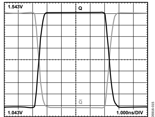
Figure 16. 50 MHz Output Voltage Waveform V CCO = 5.5 V
