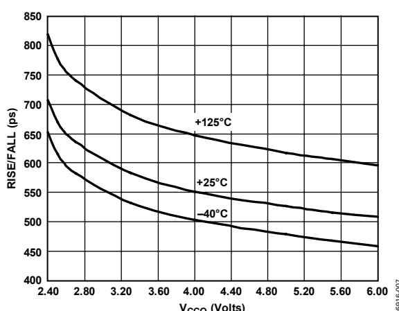
Figure 9. Output Rise/Fall Time vs. V_{CCO}
