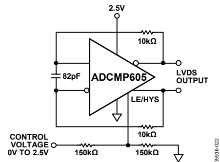
Figure 24. Voltage-Controlled Oscillator
