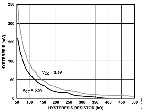
Figure 10. Hysteresis vs. R_{HYS}
