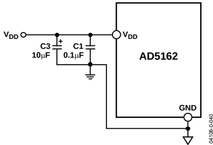
Figure 39. Power Supply Bypassing
