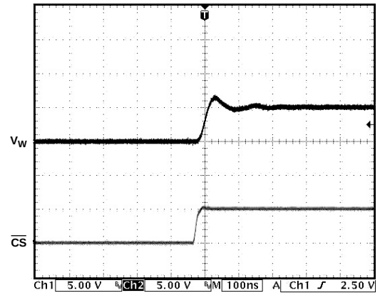
Figure 26. Large Signal Settling Time
