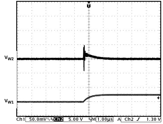
Figure 24. Analog Crosstalk
