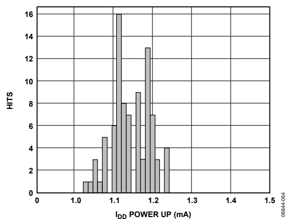
Figure 20. I_{DD} Histogram, V_{DD} = 5.0\text{ V}
