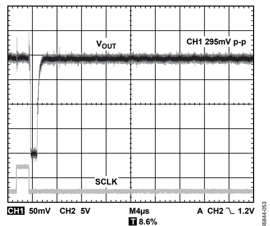
Figure 35. Glitch Upon Entering Power-Down (1 kΩ to GND) from Zero Scale, No Load
