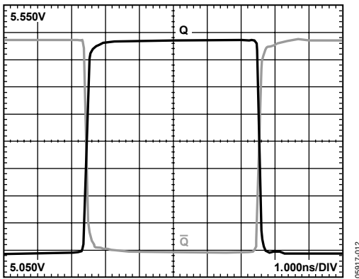
Figure 13. Output Waveform at V_{CC} = 5.5V
