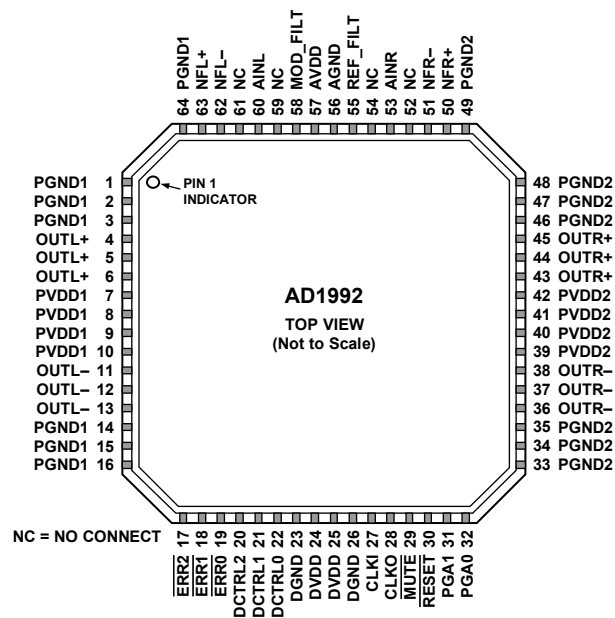
Figure 3. Pin Configuration
