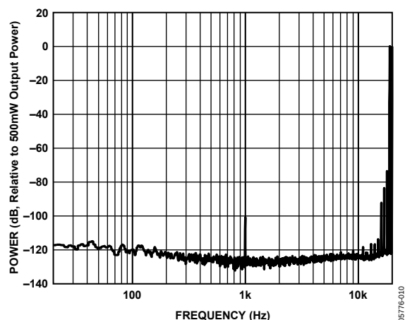
Figure 10. IMD for 19 kHz/20 kHz Twin-Tone Stimulus with 500 mW Power in Each Tone
