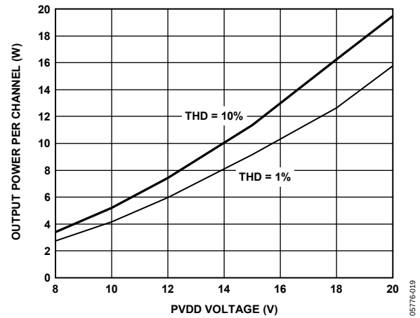
Figure 19. Maximum Output Power vs. PVDD, 4 \Omega Load
