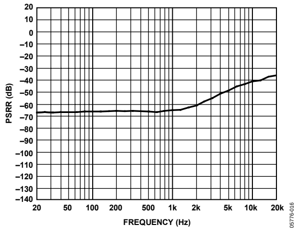
Figure 16. Power Supply Rejection Ratio (PSRR) vs. Frequency
