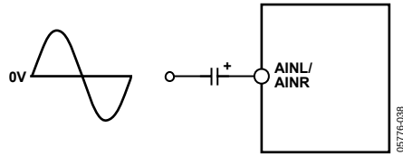
Figure 34. AC-Coupled Input Signal
