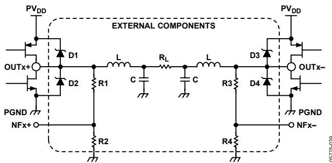
Figure 35. H-Bridge Configuration
