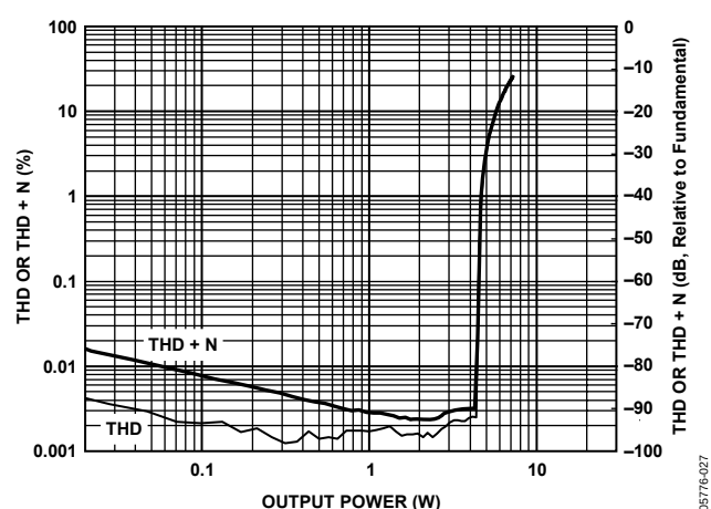
Figure 27. THD and THD + N vs. Output Power, 1 kHz Sine, 8 \Omega Load, PVDD = 15 V
