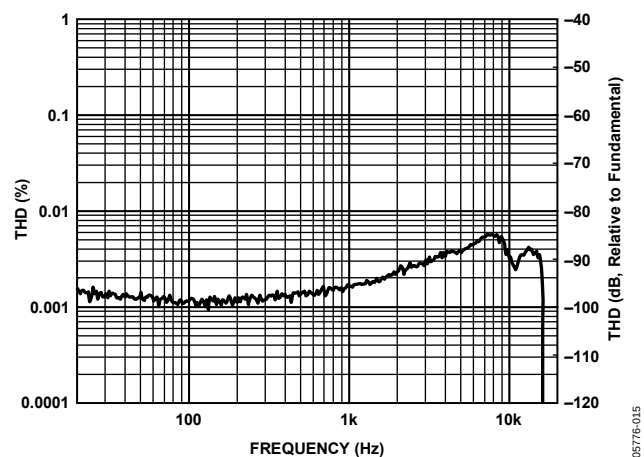
Figure 15. THD vs. Frequency, 1 W Output Power into 8 \Omega Load, PVDD = 12 V
