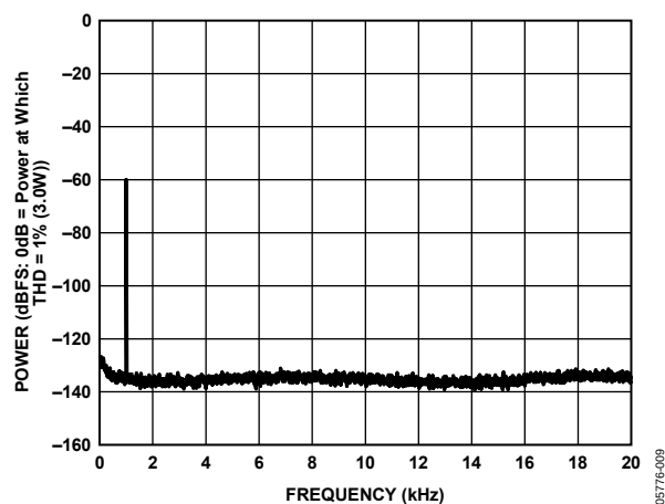
Figure 9. -60 dBFS Output Power into 8 Ω Load, PVDD = 12 V
