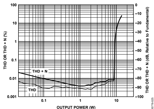
Figure 25. THD and THD + N vs. Output Power, 1 kHz Sine, 4 \Omega Load, PVDD = 15 V
