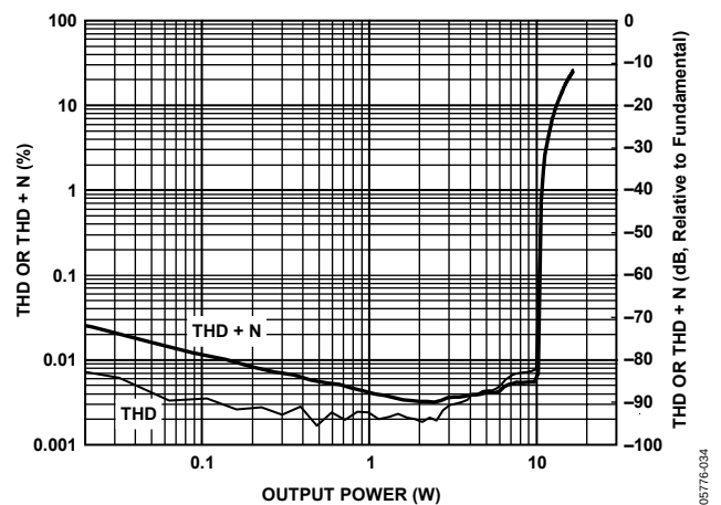
Figure 32. THD and THD + N vs. Output Power, 1 kHz Sine, 6 Ω Load, PVDD = 20 V
