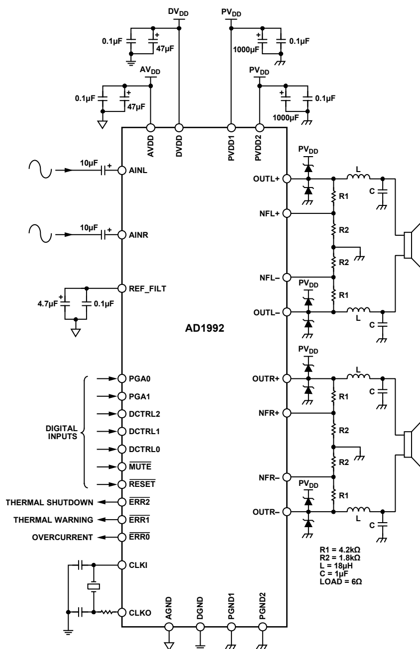
Figure 38. Typical Application Circuit
