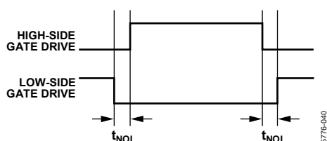
Figure 36. Half-Bridge Nonoverlap Delay Timing
