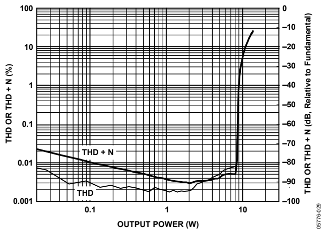
Figure 29. THD and THD + N vs. Output Power, 1 kHz Sine, 6 Ω Load, PVDD = 18 V
