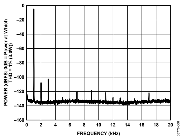
Figure 6. 1 W Output Power into 8 Ω Load, PVDD = 12 V
