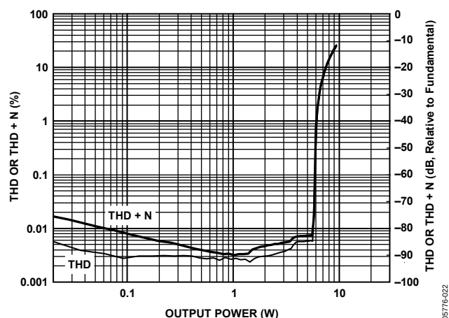
Figure 22. THD and THD + N vs. Output Power, 1 kHz Sine, 4 \Omega Load, PVDD = 12 V
