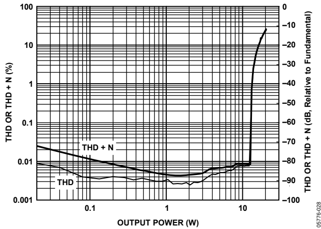
Figure 28. THD and THD + N vs. Output Power, 1 kHz Sine, 4 Ω Load, PVDD = 18 V
