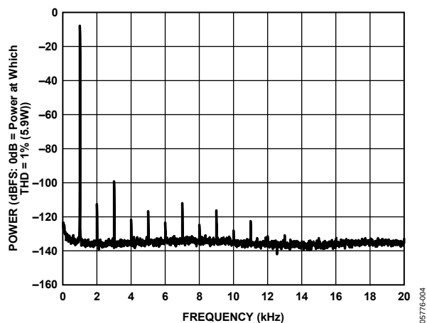
Figure 4. 1 W Output Power into 4 Ω Load, PVDD = 12 V
