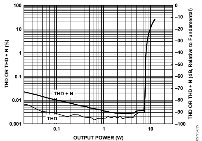
Figure 33. THD and THD + N vs. Output Power, 1 kHz Sine, 8 Ω Load, PVDD = 20 V
