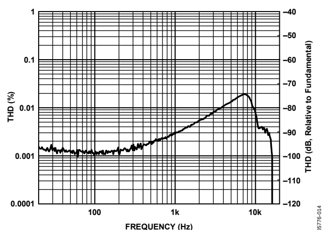
Figure 14. THD vs. Frequency, 1 W Output Power into 6 \Omega Load, PVDD = 12 V
