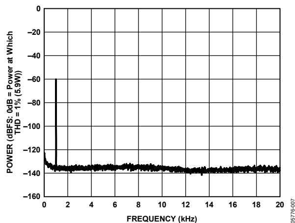
Figure 7. -60 dBFS Output Power into 4 Ω Load, PVDD = 12 V
