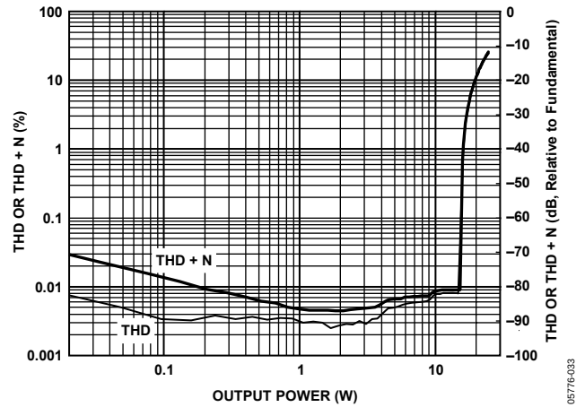
Figure 31. THD and THD + N vs. Output Power, 1 kHz Sine, 4 Ω Load, PVDD = 20 V
