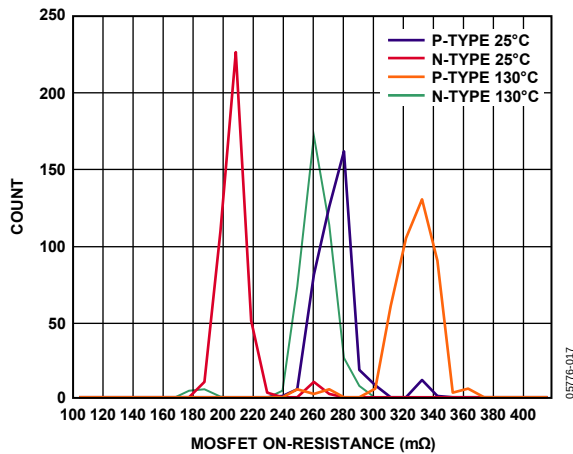
Figure 17. Histogram Showing Manufacturing Variation of R_{DS-ON} of the Output MOSFETs at 25°C and 130°C
