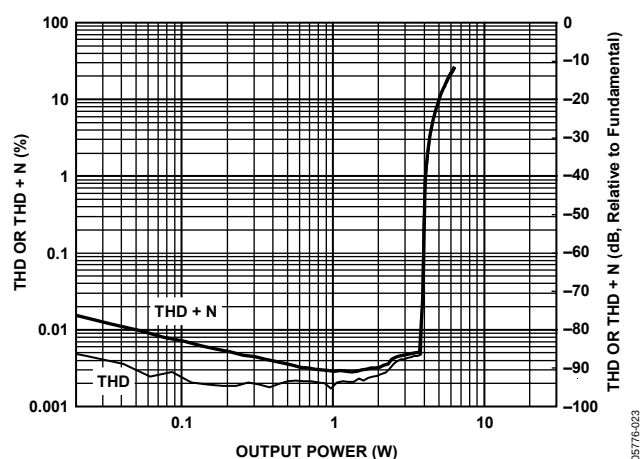
Figure 23. THD and THD + N vs. Output Power, 1 kHz Sine, 6 \Omega Load, PVDD = 12 V
