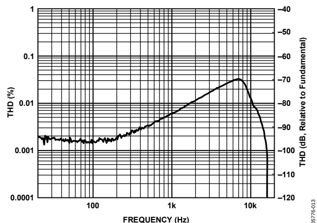
Figure 13. THD vs. Frequency, 1 W Output Power into 4 \Omega Load, PVDD = 12 V
