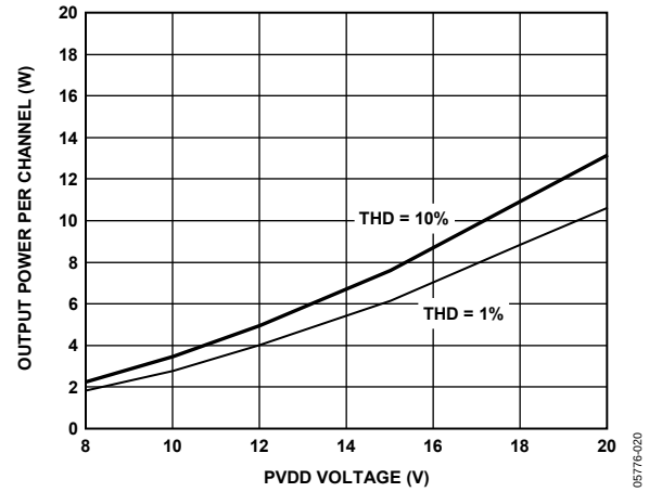
Figure 20. Maximum Output Power vs. PVDD, 6 \Omega Load
