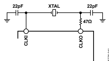
Figure 37. Crystal Connection
