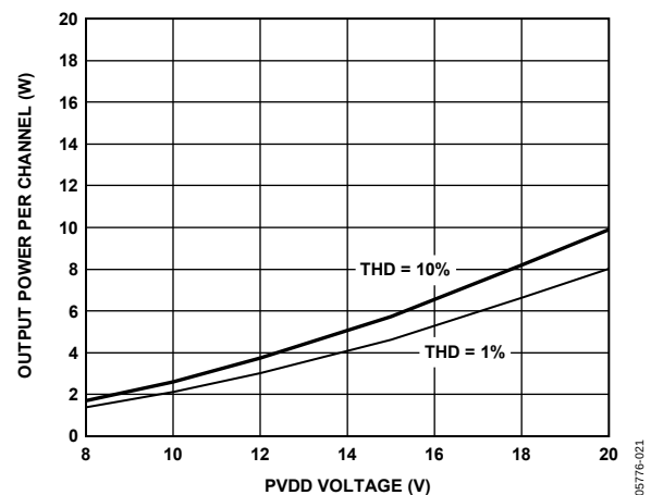
Figure 21. Maximum Output Power vs. PVDD, 8 \Omega Load
