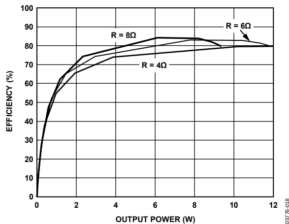
Figure 18. Efficiency vs. Output Power, PVDD = 12 V
