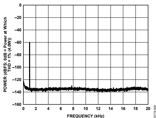
Figure 8. -60 dBFS Output Power into 6 Ω Load, PVDD = 12 V
