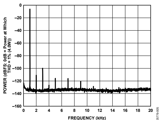
Figure 5. 1 W Output Power into 6 Ω Load, PVDD = 12 V
