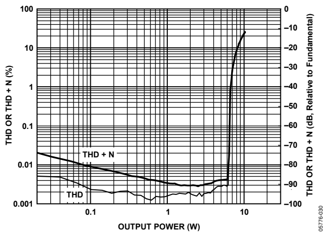
Figure 30. THD and THD + N vs. Output Power, 1 kHz Sine, 8 Ω Load, PVDD = 18 V
