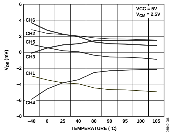
Figure 9. Offset Voltage vs. Temperature
