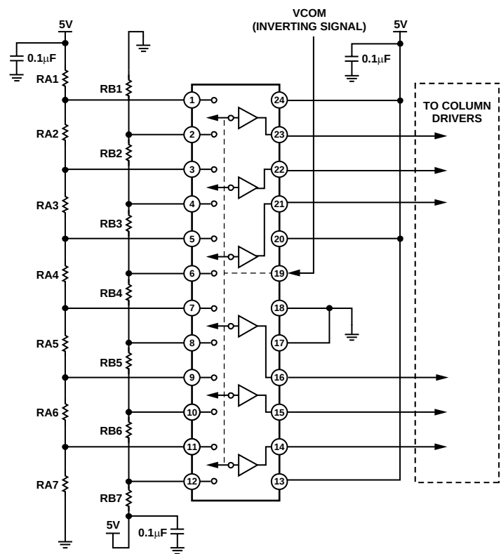
Figure 12. Typical Application
