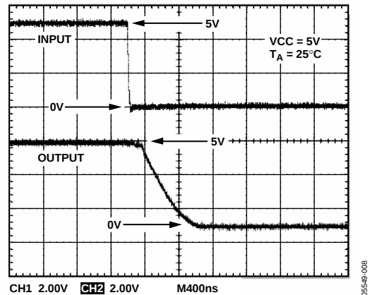
Figure 11. Transient Response—Falling
