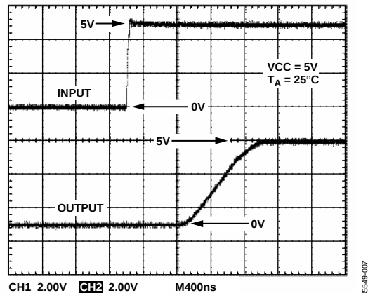
Figure 10. Transient Response—Rising
