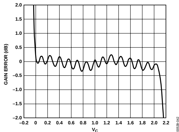
Figure 42. Gain Error for Cascaded Stages—Sequential Control
