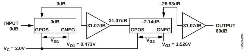
Figure 38. AD603 Gain Control Input Calculations for Sequential Operation V_C = 2.0\text{ V}
