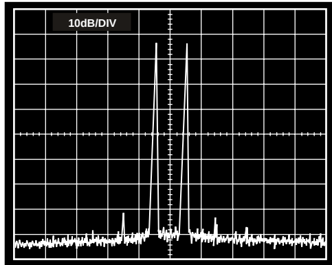
Figure 12. Third Order Intermodulation Distortion at 10.7 MHz (10x Probe Used to HP3585A Spectrum Analyzer, Gain = 0 dB, P_{IN} = 0 dBm)
