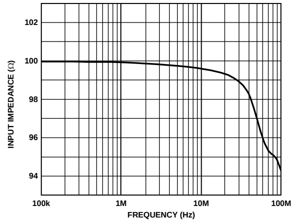
Figure 14. Input Impedance vs. Frequency (Gain = -10 dB)
