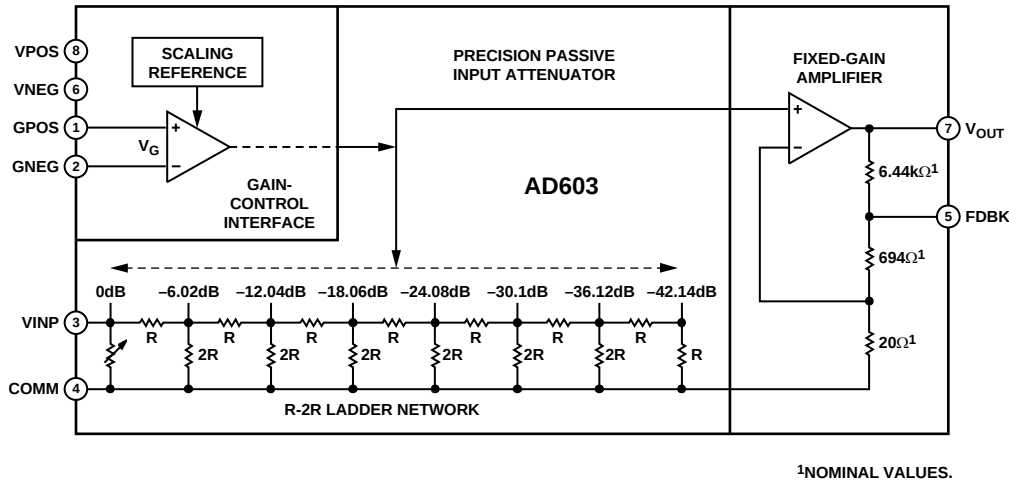
Figure 29. Simplified Block Diagram
