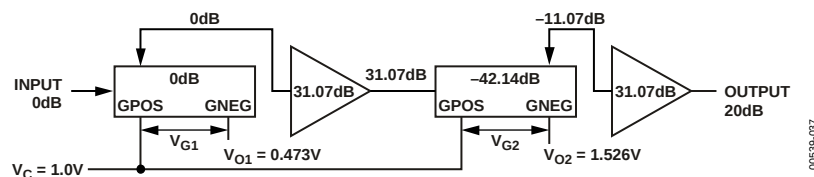
Figure 37. AD603 Gain Control Input Calculations for Sequential Control Operation V_C = 1.0 V
