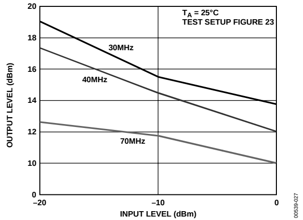
Figure 27. Third Order Intercept -10 dB/+30 dB Mode, Gain = +10 dB
