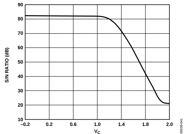
Figure 41. SNR for Cascaded Stages—Sequential Control
