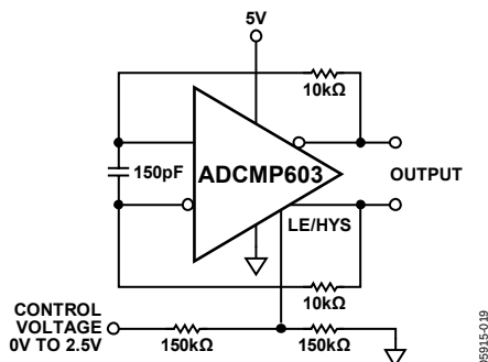
Figure 21. Voltage-Controlled Oscillator
