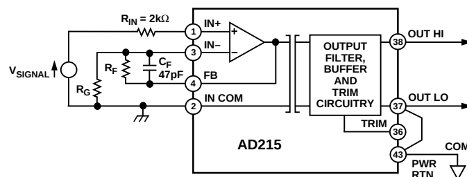
Figure 13. Noninverting Input Configuration for Gain > 1 \text{ V/V}
