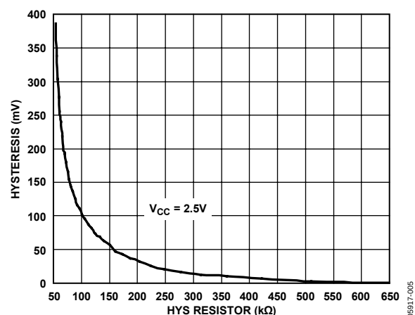
Figure 9. Hysteresis vs. R_{HYS}
