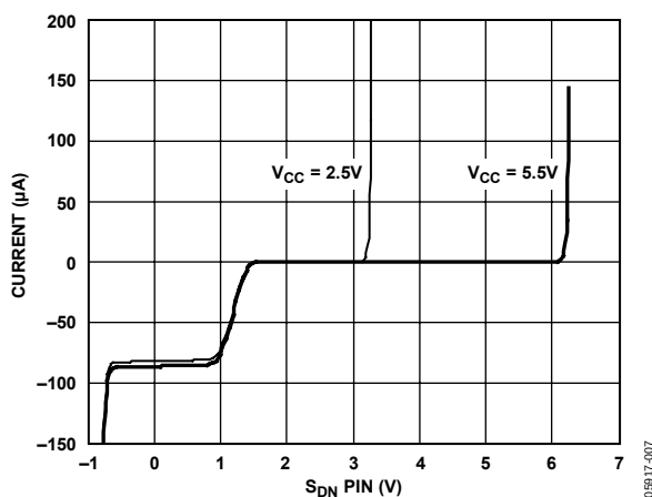
Figure 6. S_{DN} Pin I/V Curve
