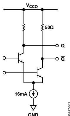
Figure 14. Simplified Schematic Diagram of CML-Compatible Output Stage
