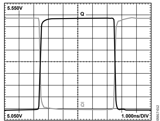
Figure 13. Output Waveform at V_{CC} = 5.5\text{ V}
