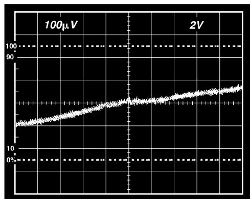
Figure 35. Gain Nonlinearity, G = 100 , R_L = 10\text{ k}\Omega ( 100\text{ }\mu\text{V} = 10\text{ ppm} )
