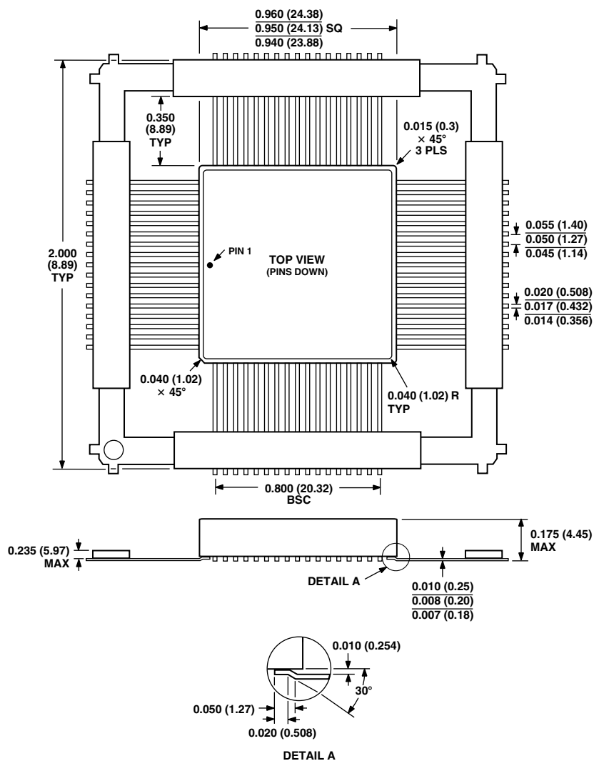
68-Lead Ceramic Leaded Chip Carrier with Nonconductive Tie-Bar (ES-68C)
