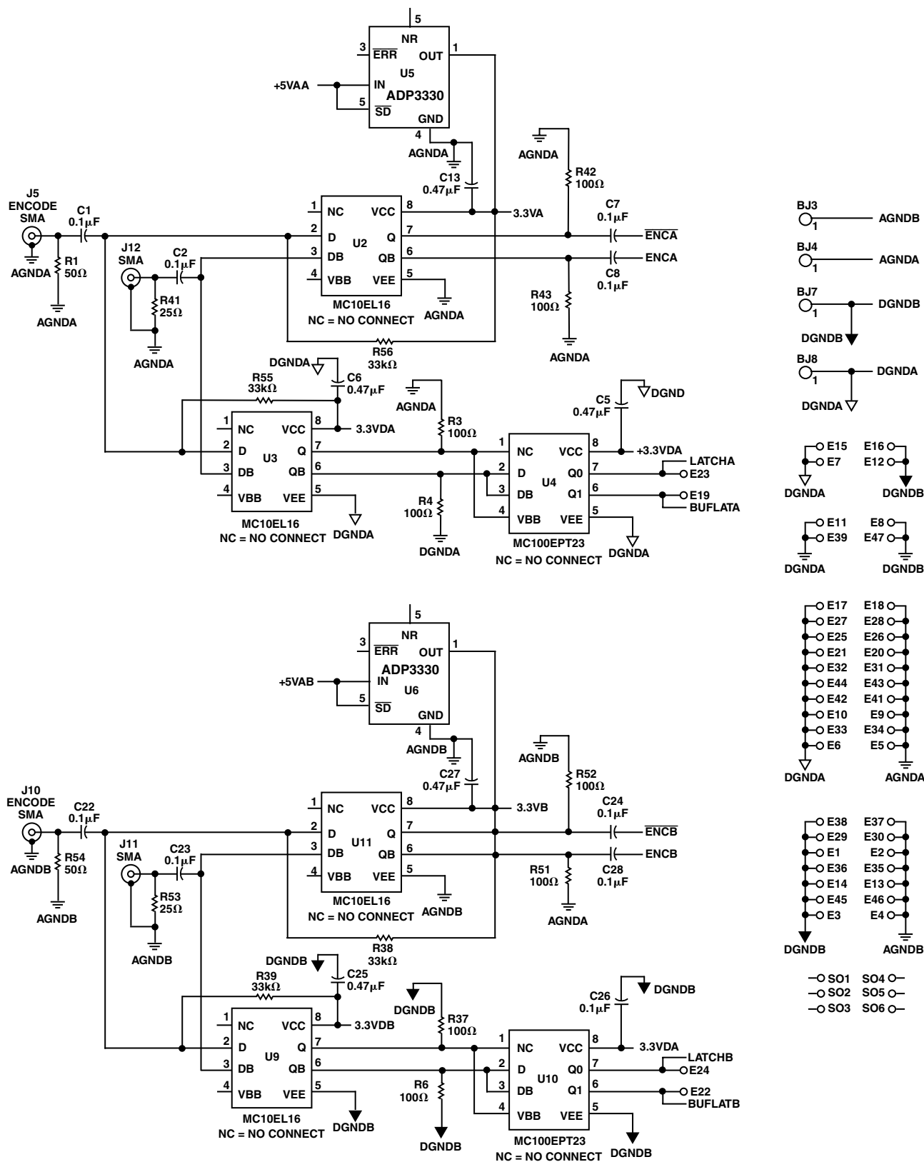
Figure 10c. Evaluation Board
