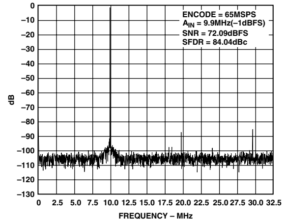
TPC 4. Single Tone @ 9.9 MHz
