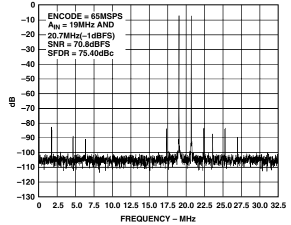
TPC 6. Two-Tone @ 19 MHz/20.7 MHz
