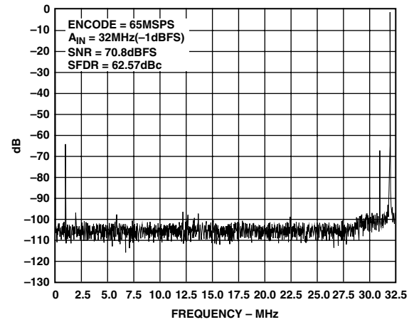
TPC 5. Single Tone @ 32 MHz
