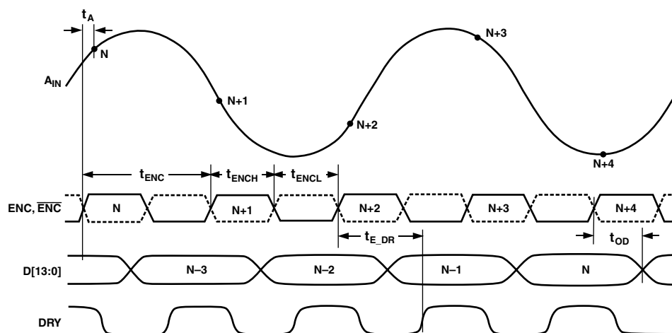
Figure 1. Timing Diagram
