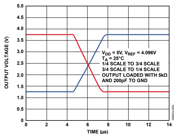
Figure 35. Typical Output Slew Rate
