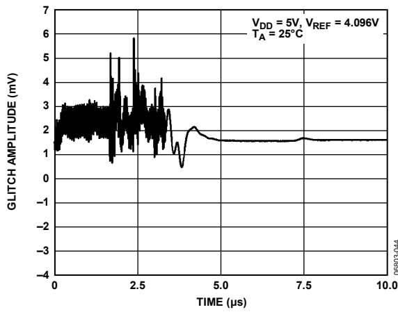
Figure 29. DAC-to-DAC Crosstalk
