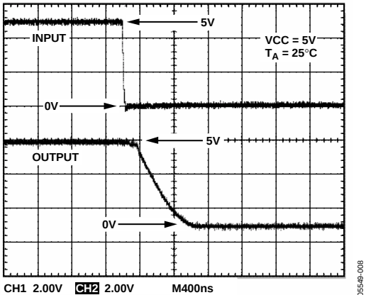
Figure 11. Transient Response—Falling
