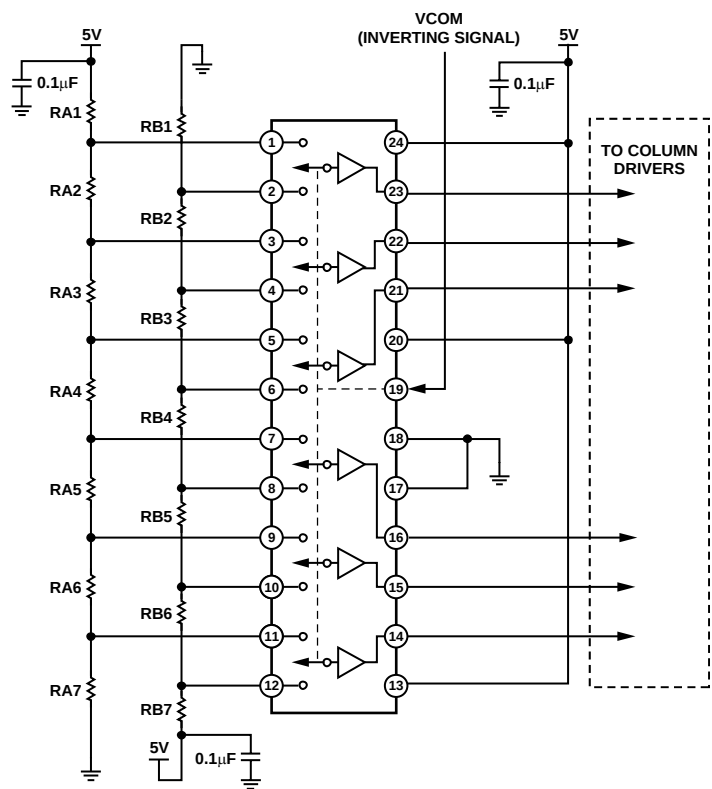
Figure 12. Typical Application
