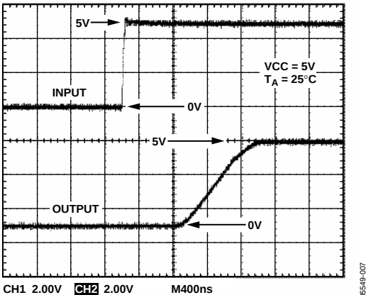
Figure 10. Transient Response—Rising
