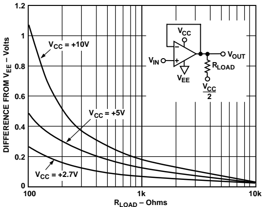
Figure 12. -Output Saturation Voltage vs. R_{LOAD} @ +85°C
