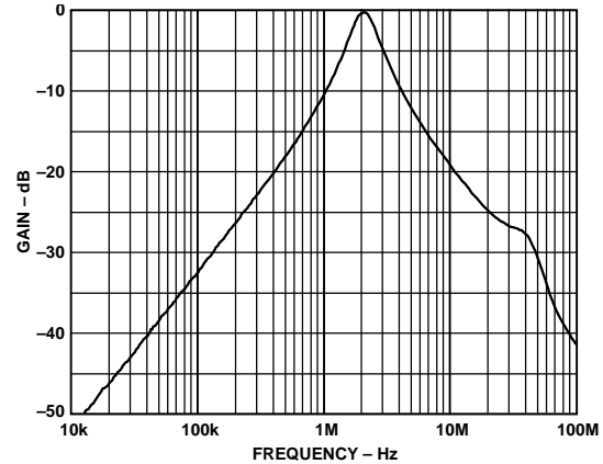
Figure 43. Frequency Response of 2 MHz Bandpass Filter
