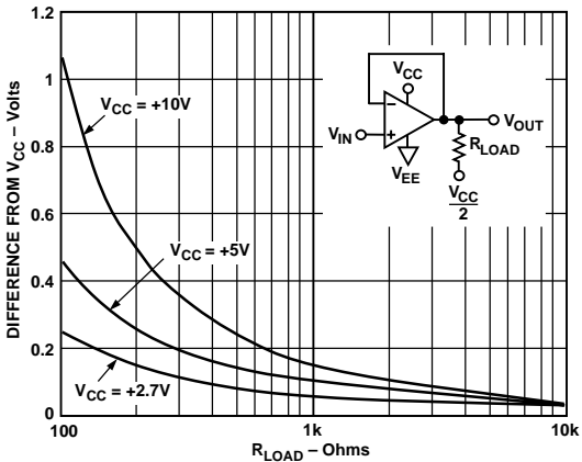
Figure 13. -Output Saturation Voltage vs. R_{LOAD} @ +25°C
