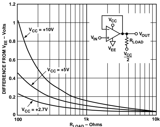
Figure 14. -Output Saturation Voltage vs. R_{LOAD} @ -40°C
