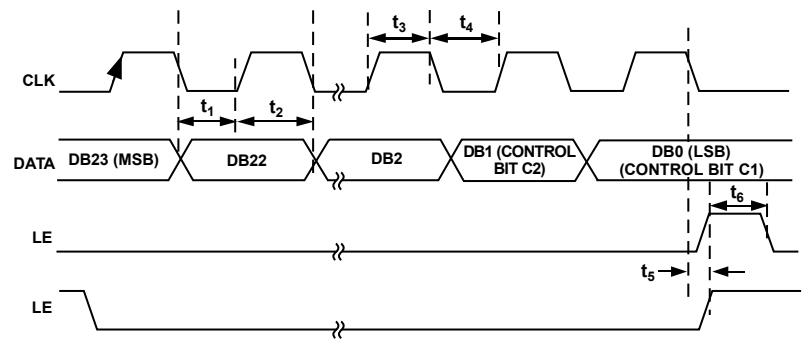
Figure 2. Timing Diagram
