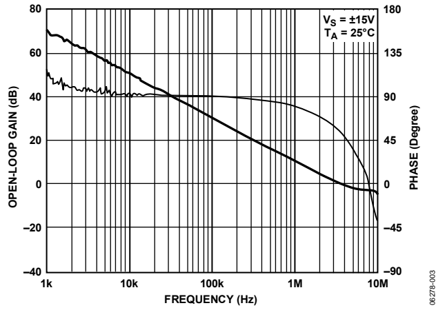
Figure 3. AD8682 Open-Loop Gain and Phase vs. Frequency
