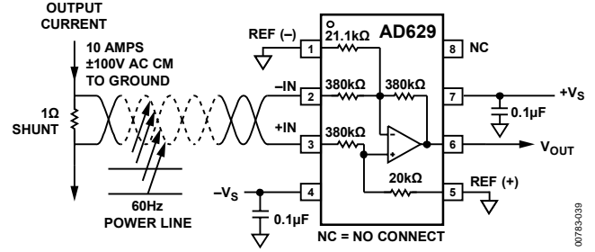
Figure 39. Error Budget Analysis Example 2: V_{IN} = 10 V Full-Scale, V_{CM} = \pm 100 V at 500 Hz, R_{SHUNT} = 1 \Omega
