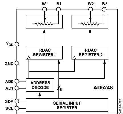
Figure 2. AD5248
