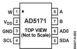
Figure 4. SOT-23-8
