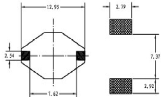
Pad Layout
