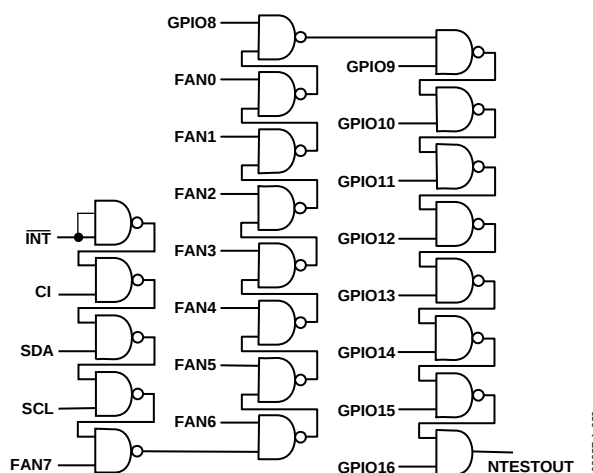
Figure 56. NAND Tree
