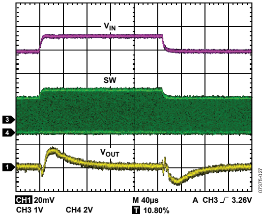
Figure 16. Line Transient, V_{OUT} = 1.8\text{ V} , PWM, 200 mA
