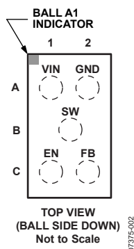
Figure 2. Pin Configuration
