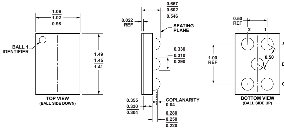
Figure 33. 5-Ball Wafer Level Chip Scale Package [WLCSP] (CB-5-3) Dimensions shown in millimeters
