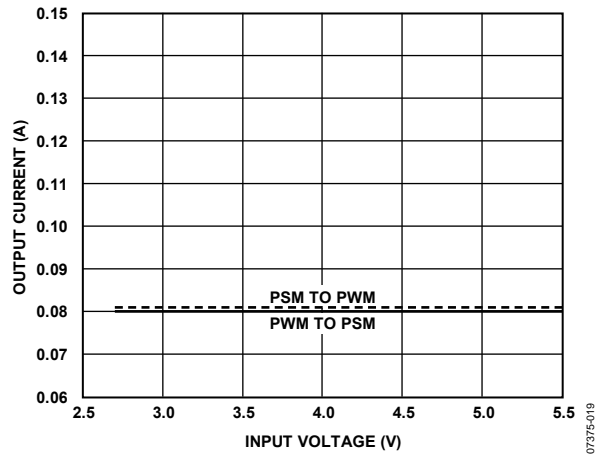
Figure 8. Mode Transition
