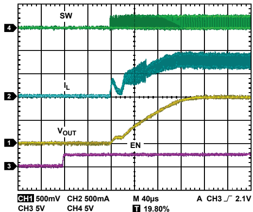
Figure 24. Start-Up, V_{OUT} = 1.0\text{ V} , 600 mA
