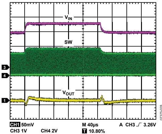
Figure 17. Line Transient, V_{OUT} = 1.0\text{ V} , PWM, 200 mA
