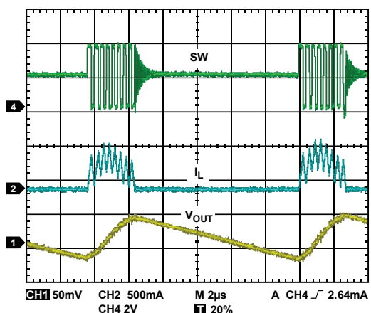
Figure 26. Typical Power Save Mode Waveform, 50 mA
