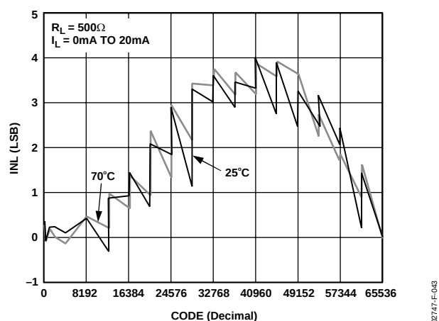
Figure 43. Result of Programmable 4 to 20 mA Current Transmitter
