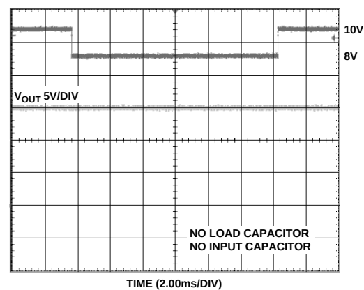
Figure 27. ADR02 Line Transient Response
