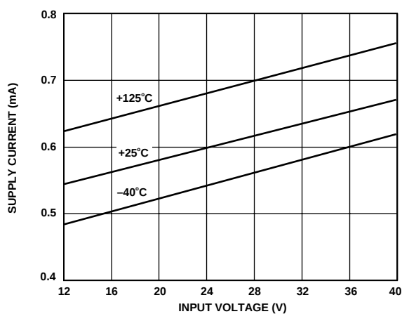
Figure 8. ADR01 Supply Current vs. Input Voltage
