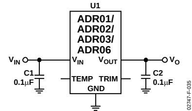
Figure 35. Basic Configuration
