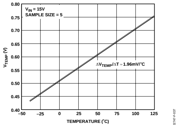
Figure 37. Voltage at TEMP Pin vs. Temperature
