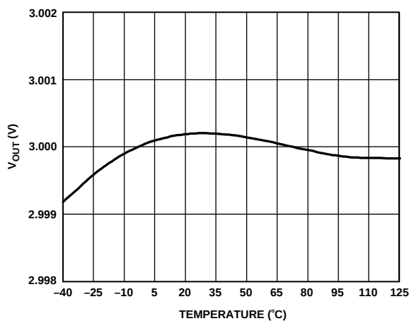
Figure 7. ADR06 Typical Output Voltage vs. Temperature
