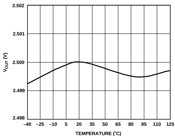
Figure 6. ADR03 Typical Output Voltage vs. Temperature
