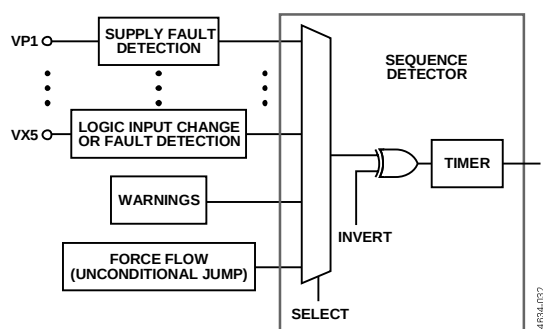
Figure 22. Sequence Detector Block Diagram
