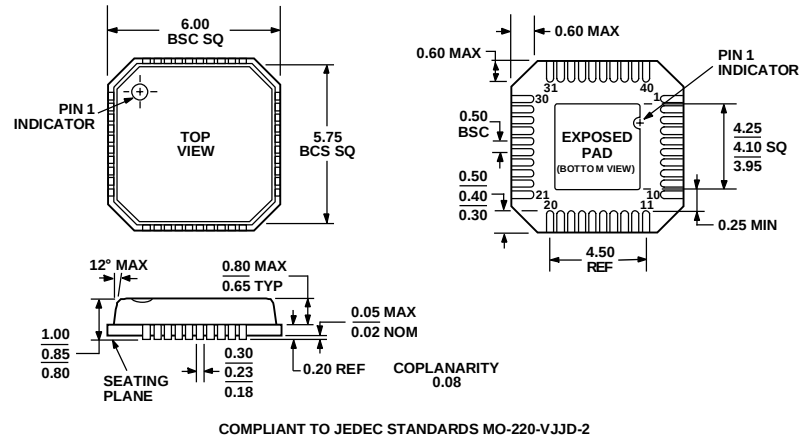
Figure 38. 40-Lead Lead Frame Chip Scale Package [LFCSF] (CP-40) Dimensions shown in millimeters
