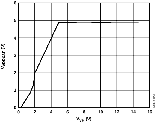
Figure 6. V_{DDCAP} vs. V_{VH}
