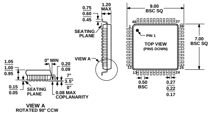
Figure 39. 48-Lead Thin Plastic Quad Flat Package [TQFP] (SU-48) Dimensions shown in millimeters
