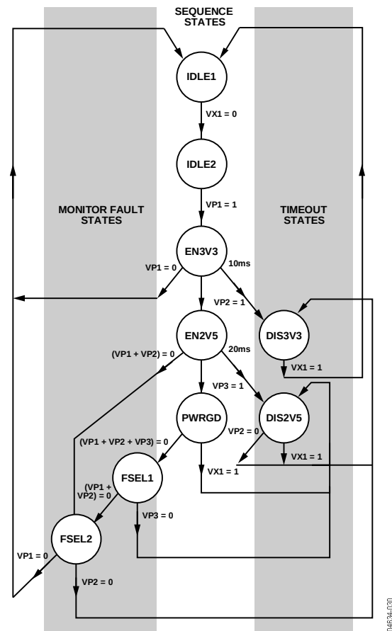
Figure 21. Sample Application Flow Diagram
