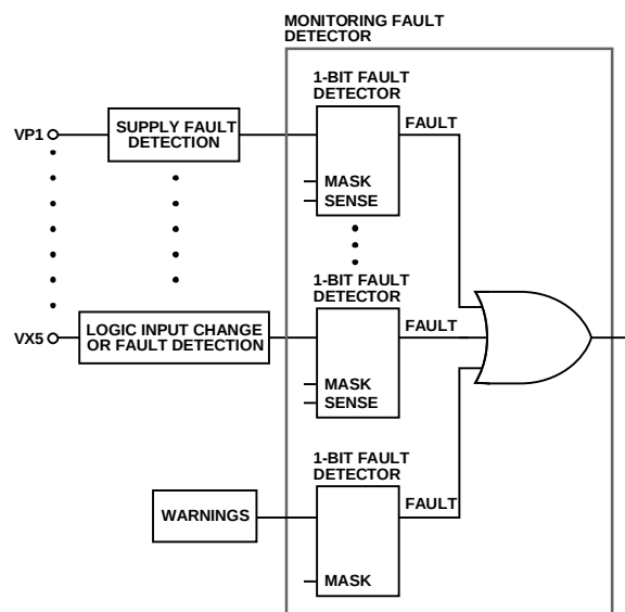
Figure 23. Monitoring Fault Detector Block Diagram
