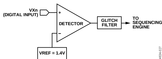
Figure 18. VXn Digital Input Function
