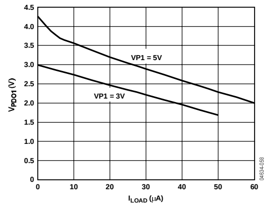
Figure 13. V_{PDO1} (Weak Pull-Up to VP ) vs. I_{LOAD}
