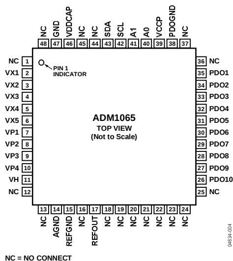
Figure 4. TQFP Pin Configuration
