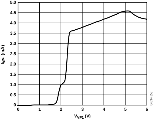
Figure 7. I_{VP1} vs. V_{VP1} (VP1 as Supply)
