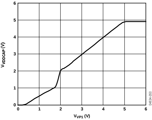
Figure 5. V_{DDCAP} vs. V_{VP1}
