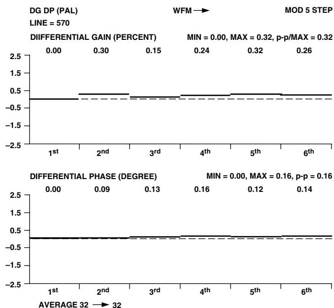
Figure 124. PAL DG DP Measurement
