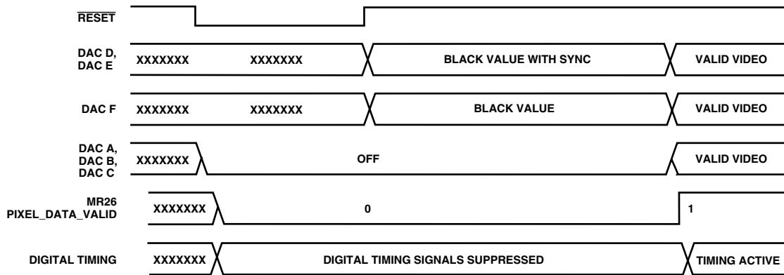
Figure 37. \overline{RESET} Sequence Timing Diagram
