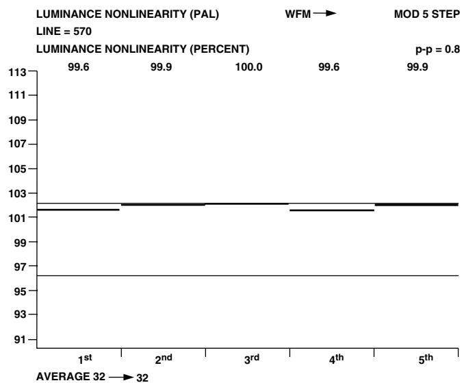
Figure 125. PAL Luminance Nonlinearity
