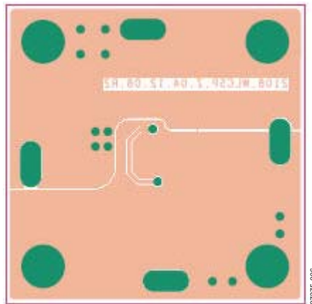
Figure 32. Recommended Bottom Layer
