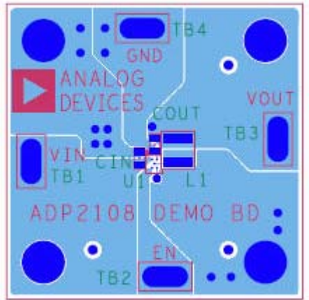
Figure 31. Recommended Top Layer
