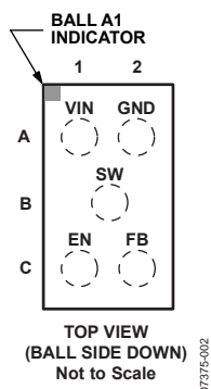
Figure 2. Pin Configuration
