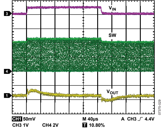
Figure 18. Line Transient, V_{OUT} = 3.3\text{ V} , PWM, 200 mA
