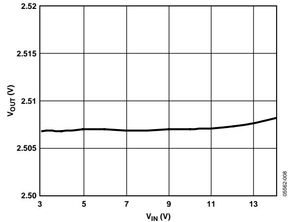
Figure 9. Typical Line Regulation vs. V_{IN} ( I_{LOAD} = 1\text{ A} ; See Figure 19)
