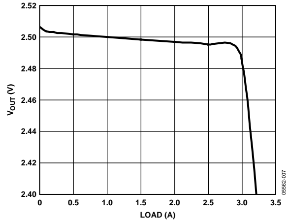
Figure 8. Typical Load Regulation ( V_{IN} = 5\text{ V} ; See Figure 1)
