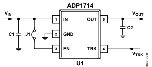
Figure 6. ADP1714 Fixed Output with Tracking
