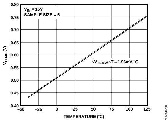
Figure 37. Voltage at TEMP Pin vs. Temperature
