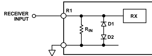
Figure 24a. Receiver Input Protection Scheme
