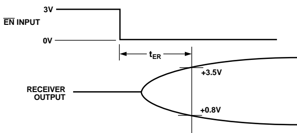
NOTE: EN IS THE COMPLEMENT OF \overline{\text{EN}} FOR THE ADM213E
