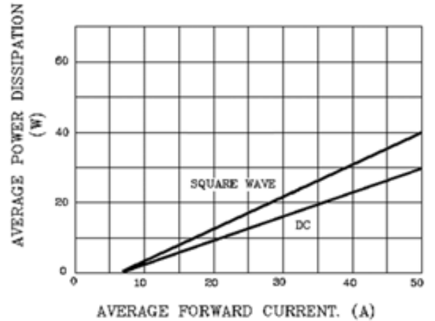
FIG.4- FORWARD POWER DISSIPATION
