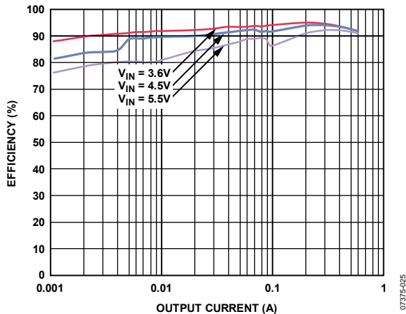
Figure 14. Efficiency, V_{OUT} = 3.3 V
