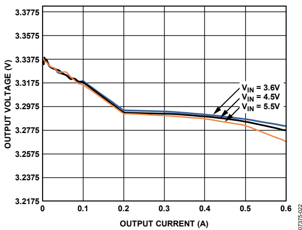
Figure 11. Load Regulation, V_{OUT} = 3.3 V
