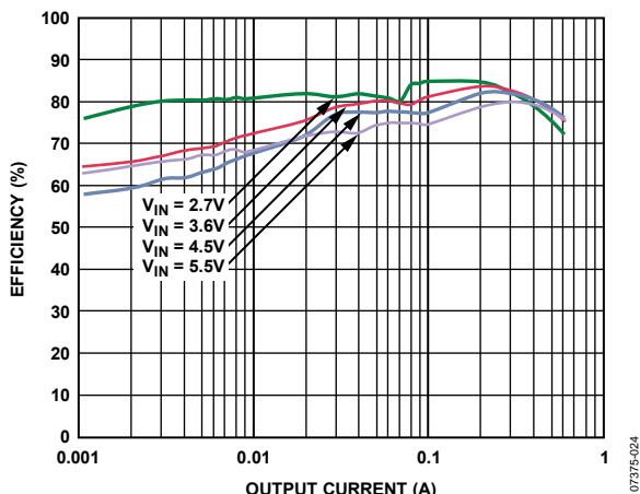
Figure 13. Efficiency, V_{OUT} = 1.0 V
