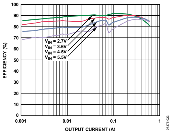
Figure 12. Efficiency, V_{OUT} = 1.8 V
