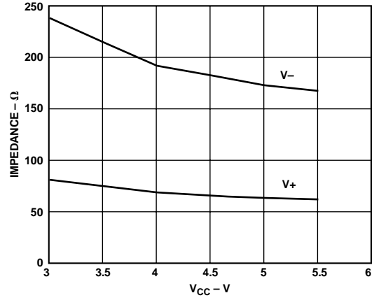
Figure 18. Charge Pump Impedance vs. V CC
