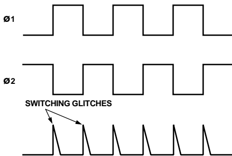
Figure 31. Switching Glitches
